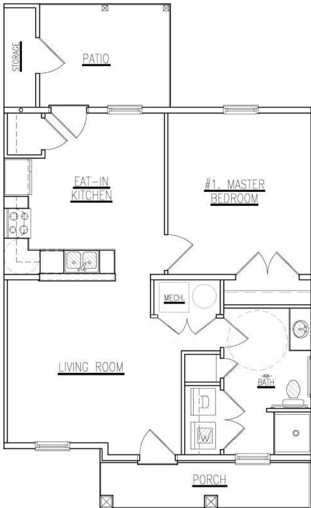
FIRST FLOOR APARTMENT 1 BEDROOM, 1 BATHROOM (Handicap Accessible)
